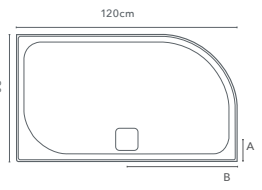
Offset Quadrant Tray
